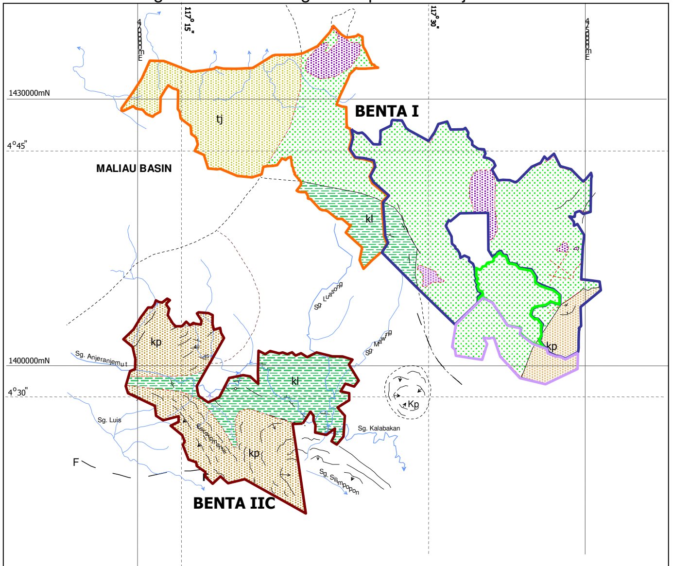
Figure A 1.1: Geological Map of the Project Area
